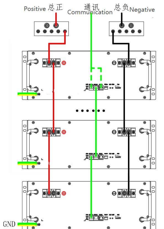
Figure 15-1 Parallel connection diagram of battery box
